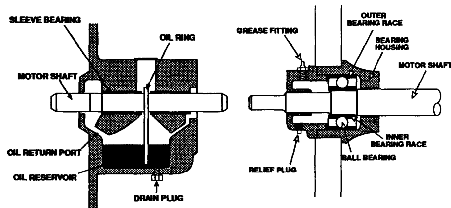
FIGURE 6-7 Sleeve Bearings Lubricated by Oil (left) and Ball Bearings Lubricated by Grease (right)
