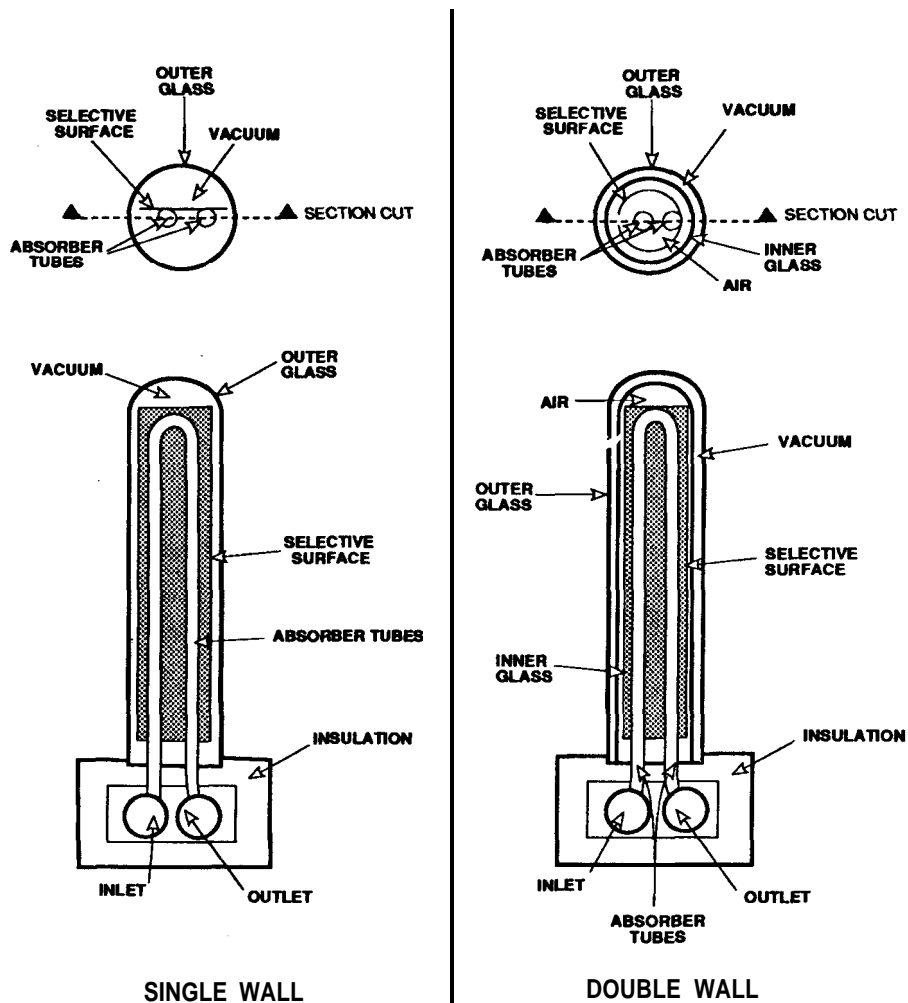
FIGURE 2-18 Single and Double Wall Evacuated Tube Collectors
