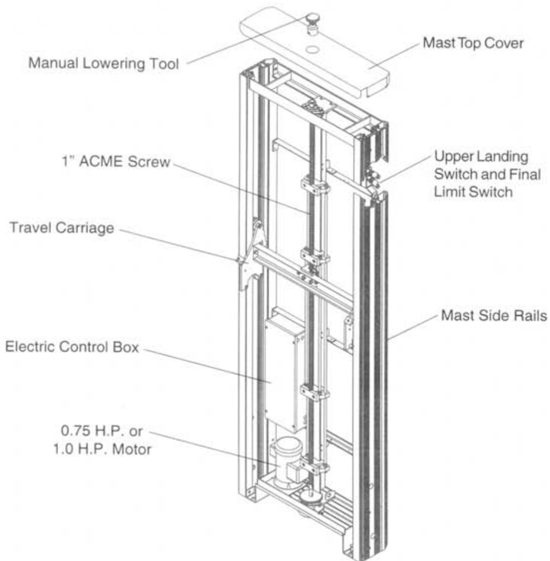
Fig. 4 - Drive System
