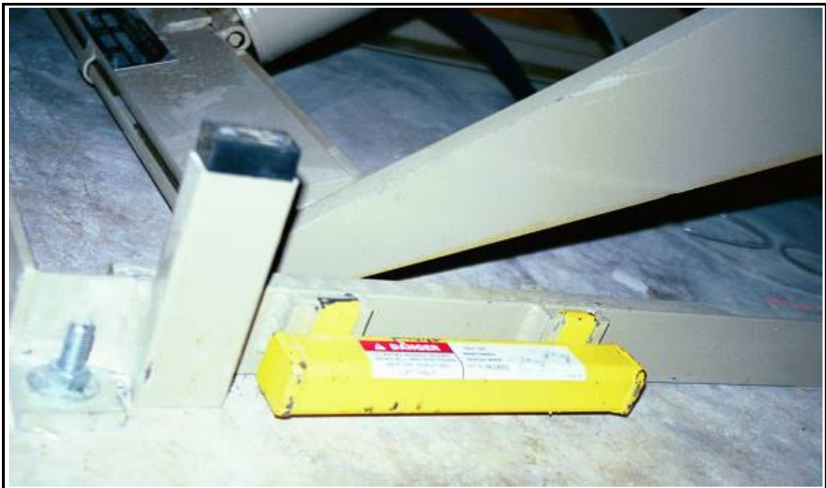
Bar To Secure Lift In Raised Position For Servicing
