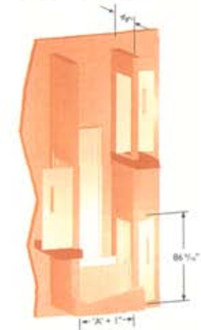
PAL-S - 168 In a hoistway with 3 fire rated doors, with a thru cab in a pit
