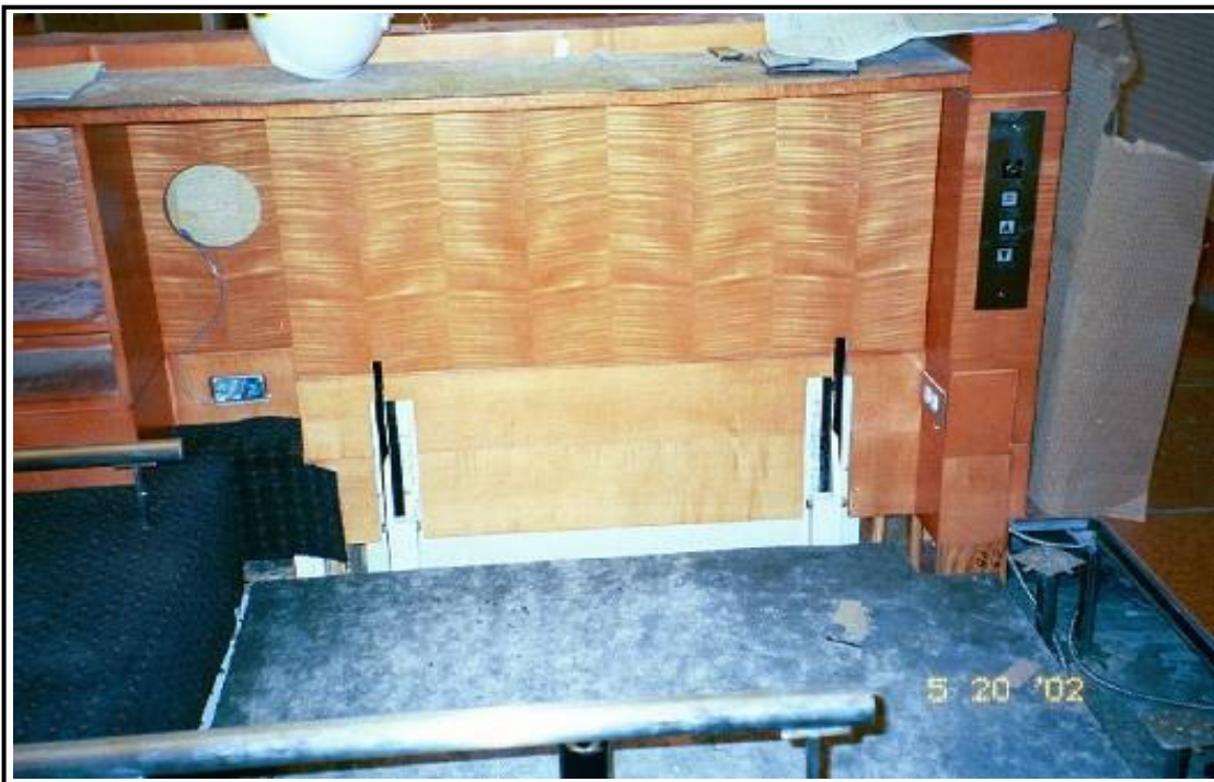
Upper Enclosure Panel Incorporated Into Millwork
