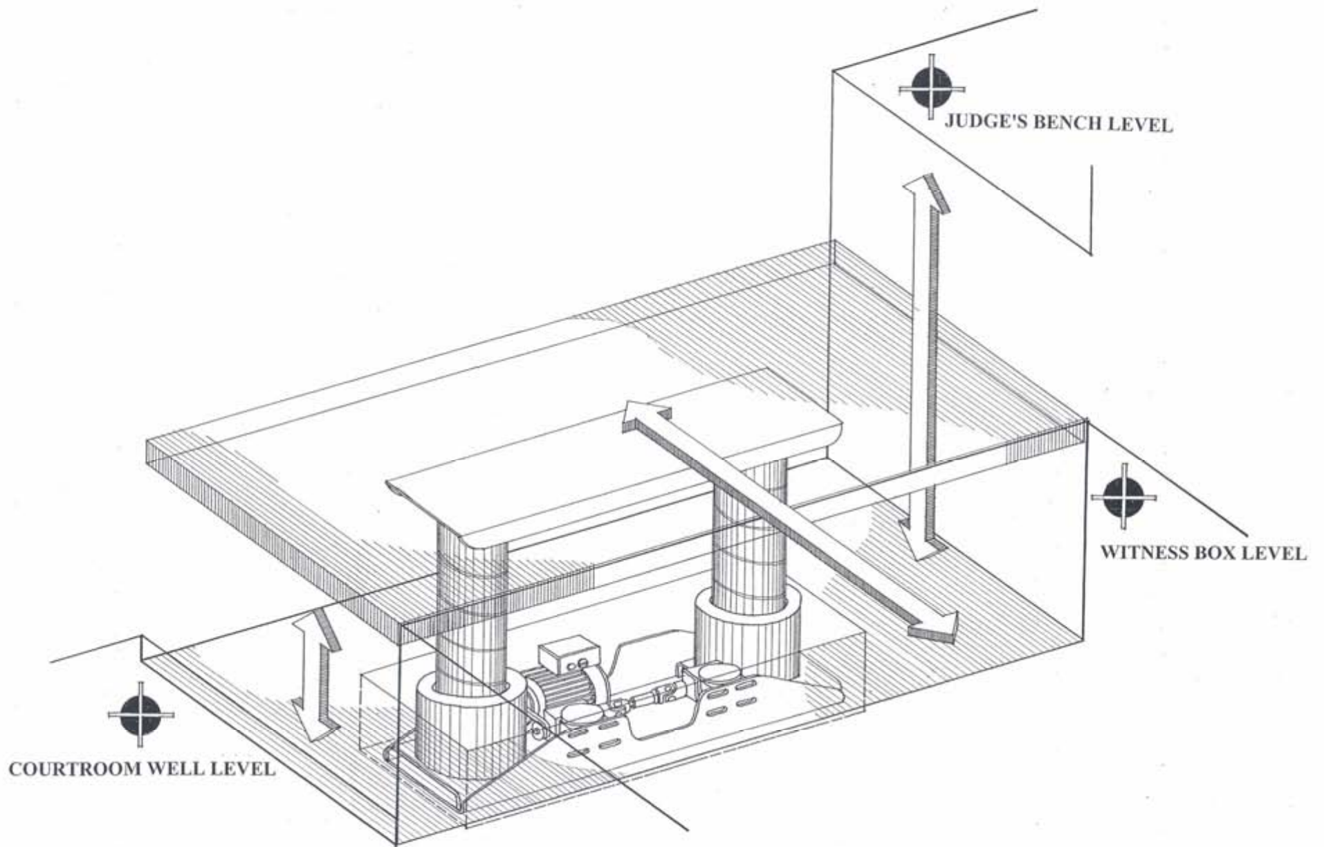
Spiralift Tandem SR Courthouse Application
