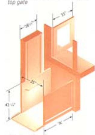
PAL-S - 72 2 Stop, thru cab with flip up ramp and top gate with no pit
