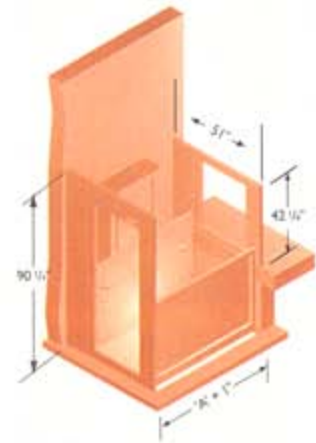
PAL-S - 48 2 stop, 36" of travel in a hoistway, in a pit, with full bottom door and top gate
