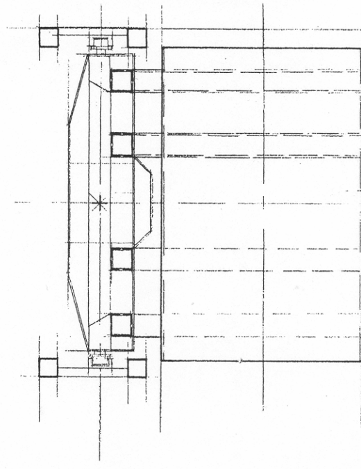
PLAN SHOWING CANILEVERED FRAME ATTACHED TO THE SPIRALIFT SUPPORTING THE PLATFORM
