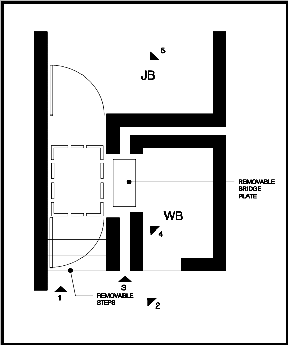
PLAN DIAGRAM AT LIFT LOCATIONS (WITNESS BOX / JUDGE'S BENCH)
