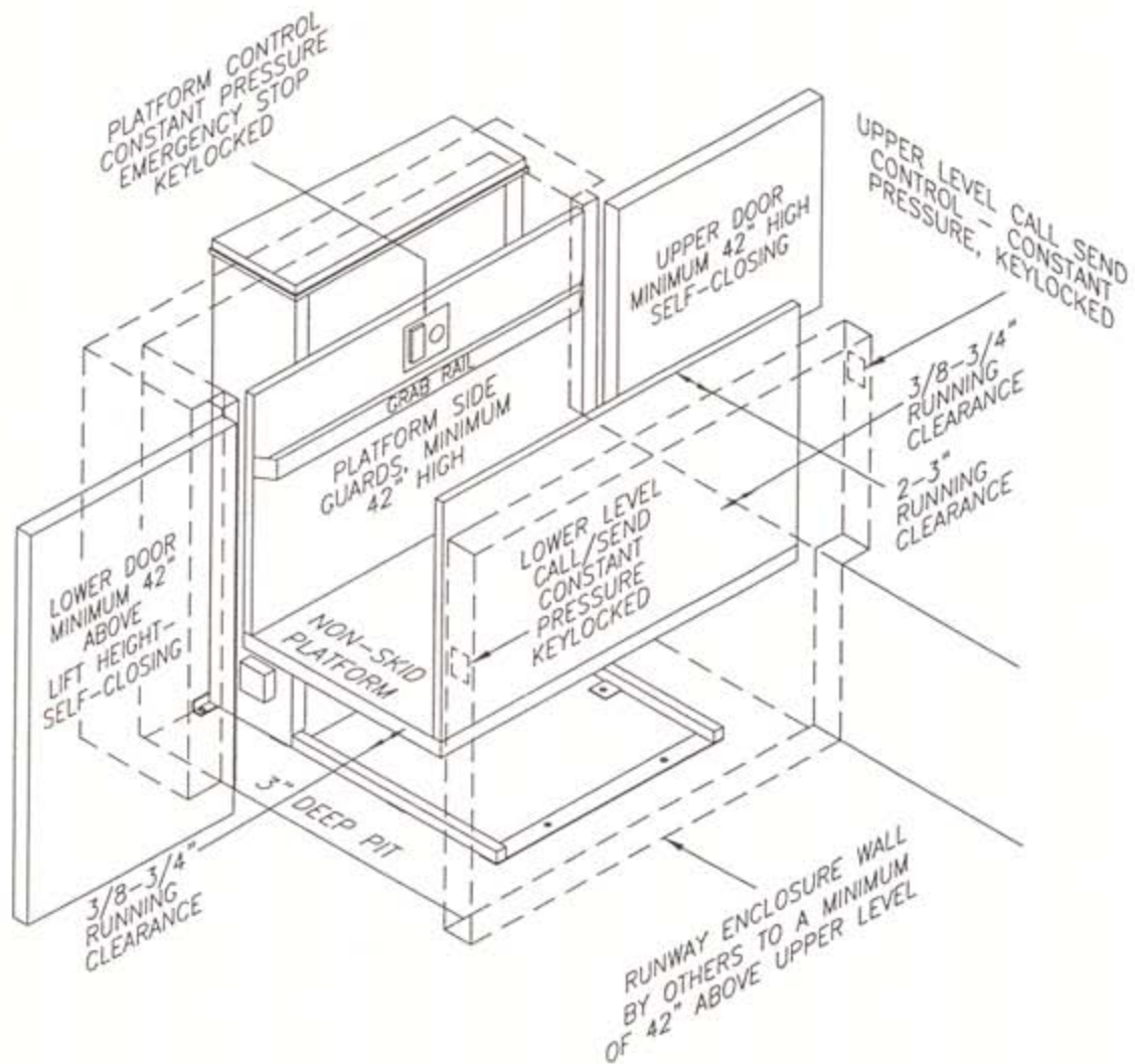
TYPICAL VERTICAL WHEELCHAIR LIFT
