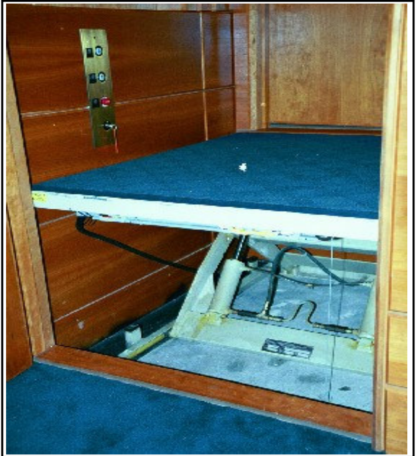
Controls Too Low At Elevated Lift Position
