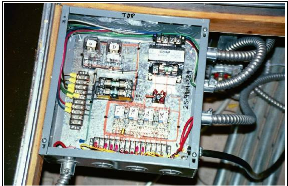
System Electrical Panel
