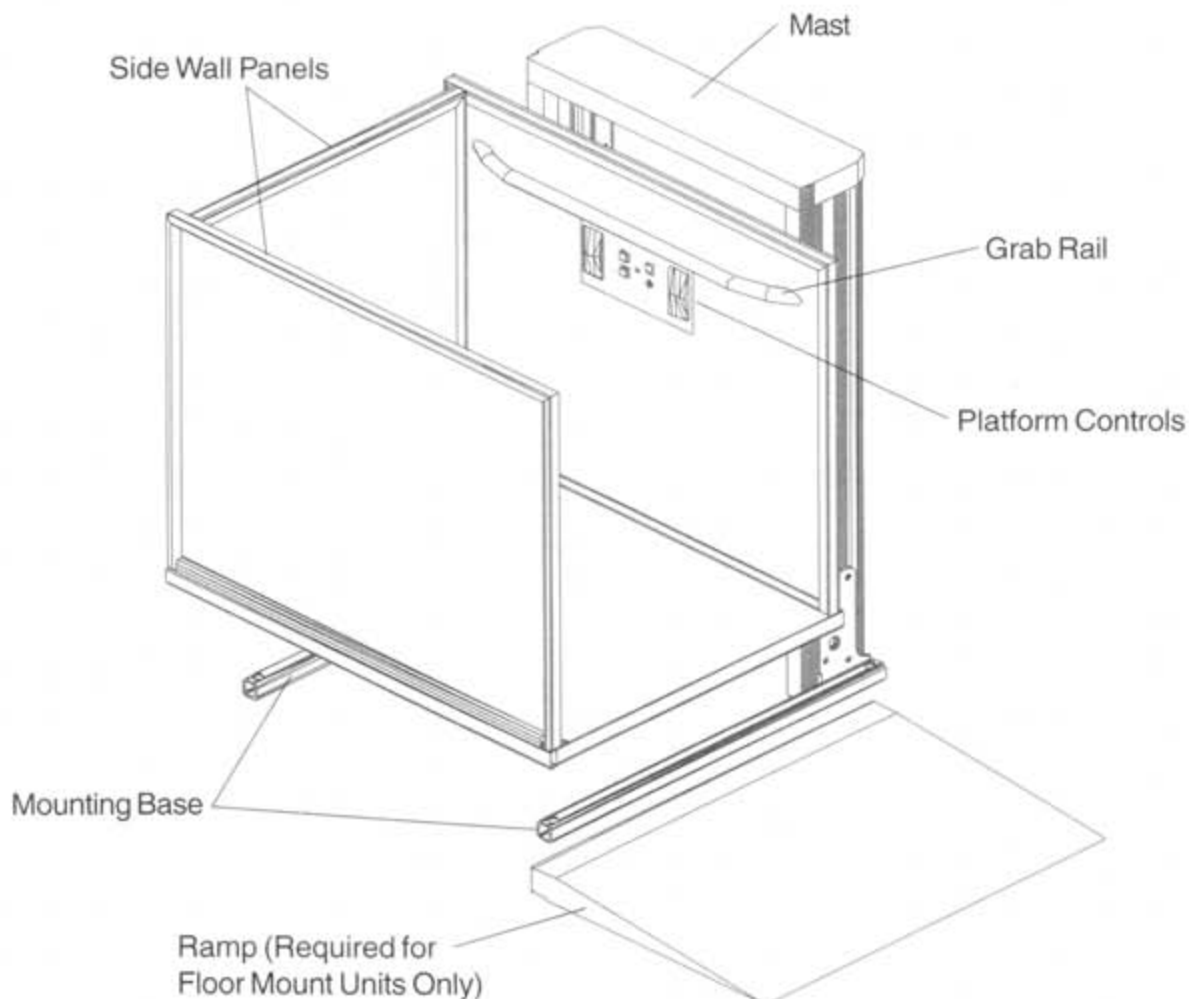
Fig. 1 - On/Off Same Side (Adjacent to Mast) Configuration
