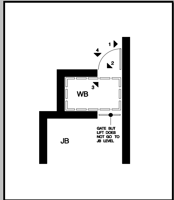
PLAN DIAGRAM AT LIFT LOCATIONS
