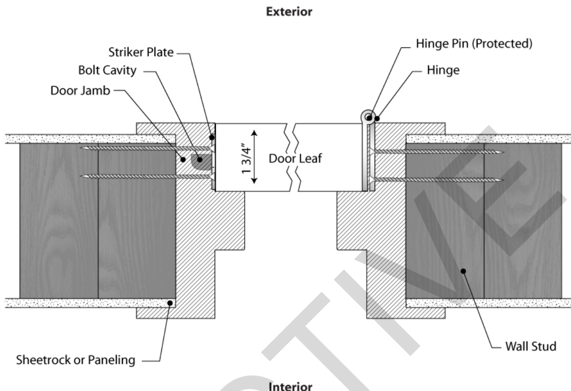
FIGURE 7-2. TOP VIEW DOOR FRAME SYSTEM
