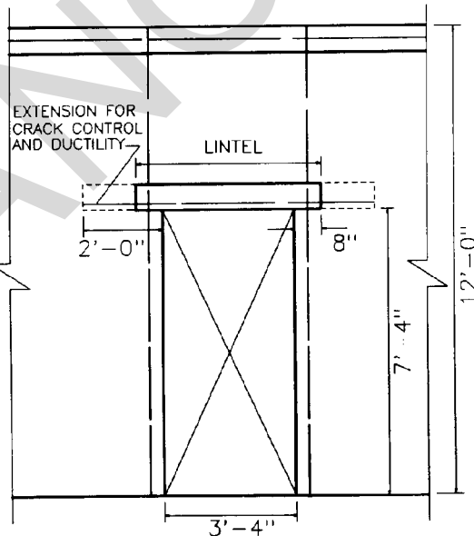
Figure 8-2. Example 1 wall elevation.
