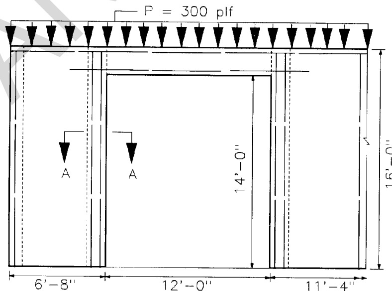
Figure 6-3. Example 3 wall elevation.
