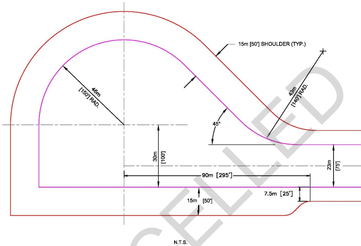
Figure 6-31. Typical Hazardous Cargo Pad for APOE/Ds
