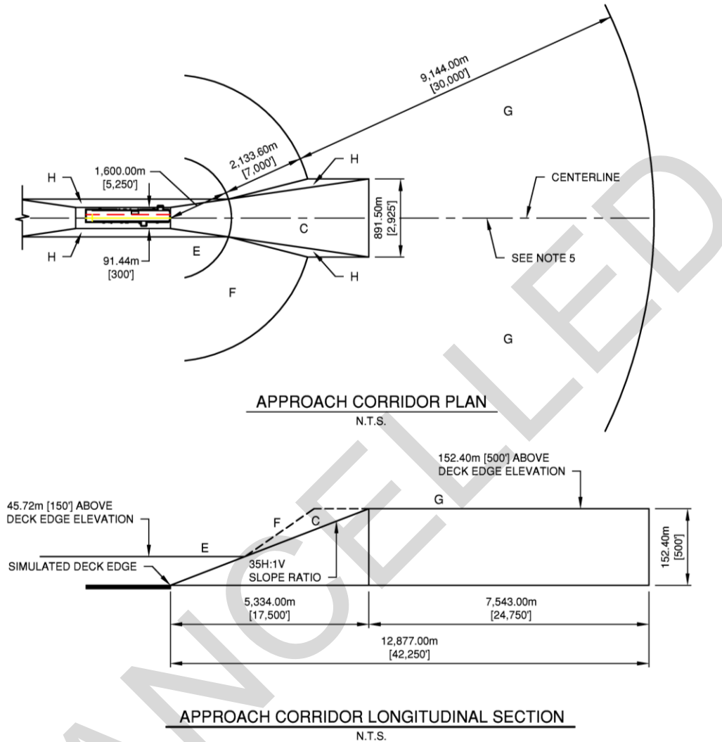
Figure 8-9. LHD STOVL Facility Approach Path Imaginary Surfaces
