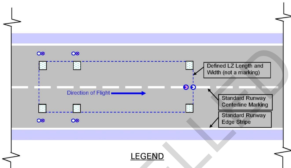
Figure 7-15. AMP-3 Lighting and Marking Scheme for LZ Superimposed on Class A or B Runway
