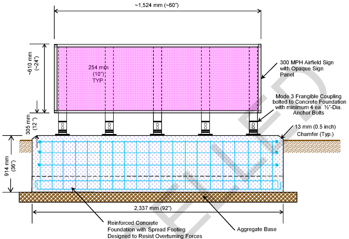
Figure 7-7. Example VLZMP on Concrete Base Detail
