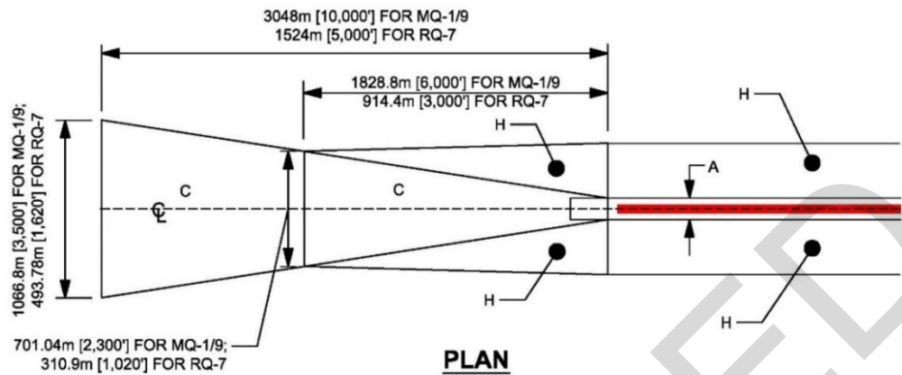
Figure 9-6. MQ-1/9 & RQ-7Bv2 Runway Plan and Profile Airspace Imaginary Surfaces
