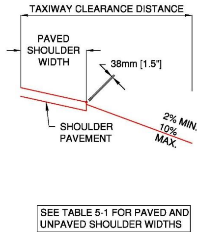
EDGE OF TAXIWAY FOR CLASS A RUNWAYS AND CLASS B RUNWAYS FOR B-52 AIRCRAFT N.T.S.
