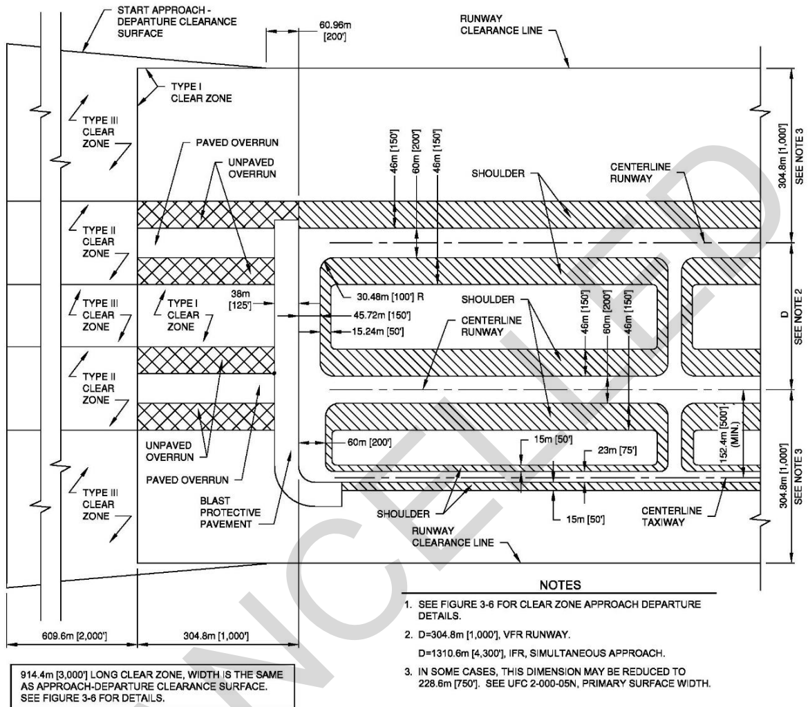
Figure 3-22. Typical Layout, Navy Dual Class B Runways
