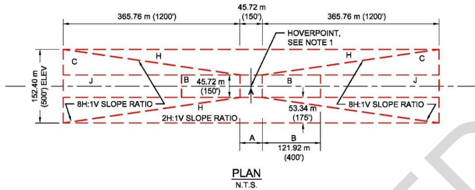
Figure 4-14. Helicopter Hoverpoint
