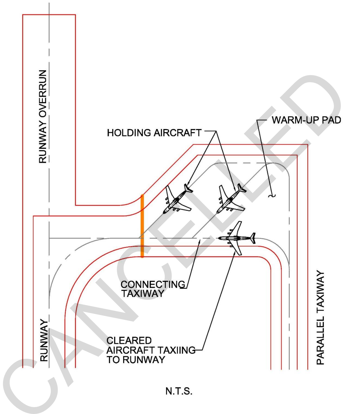
Figure 6-13. Warm-Up Pad at End of Parallel Taxiway
