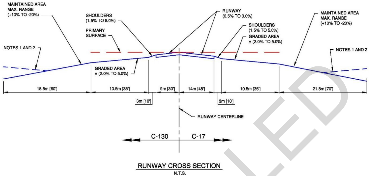
Figure 7-6. LZ Runway, Taxiway, and Apron Sections
