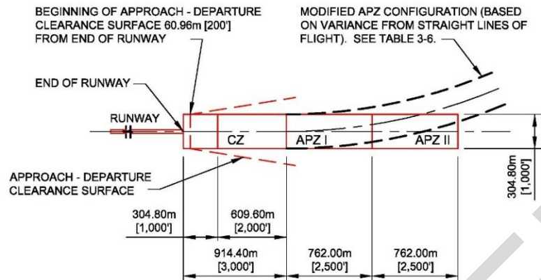
NAVY AND MARINE CORPS CLASS A RUNWAY N.T.S.
