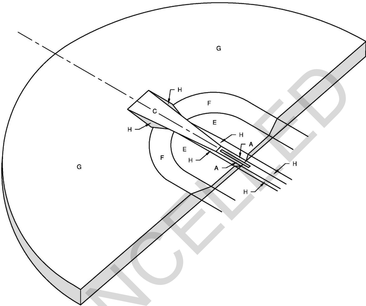
Figure 8-7. LHD STOVL Facility Departure Surface Isometric View
