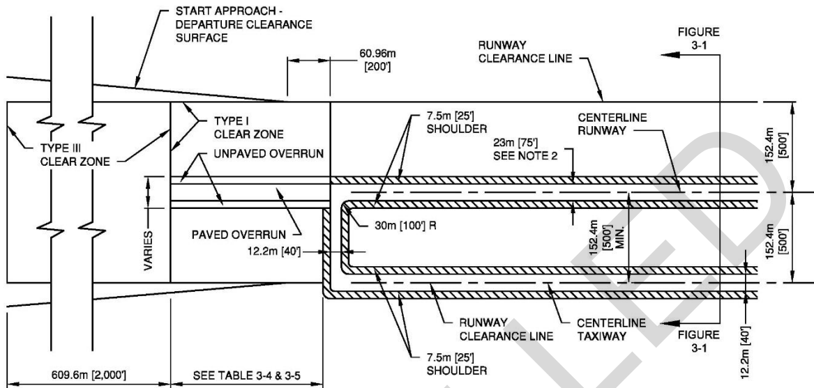
Figure 3-20. Plan, Single Runway, Navy Class A, and Basic Training Outlying Field
