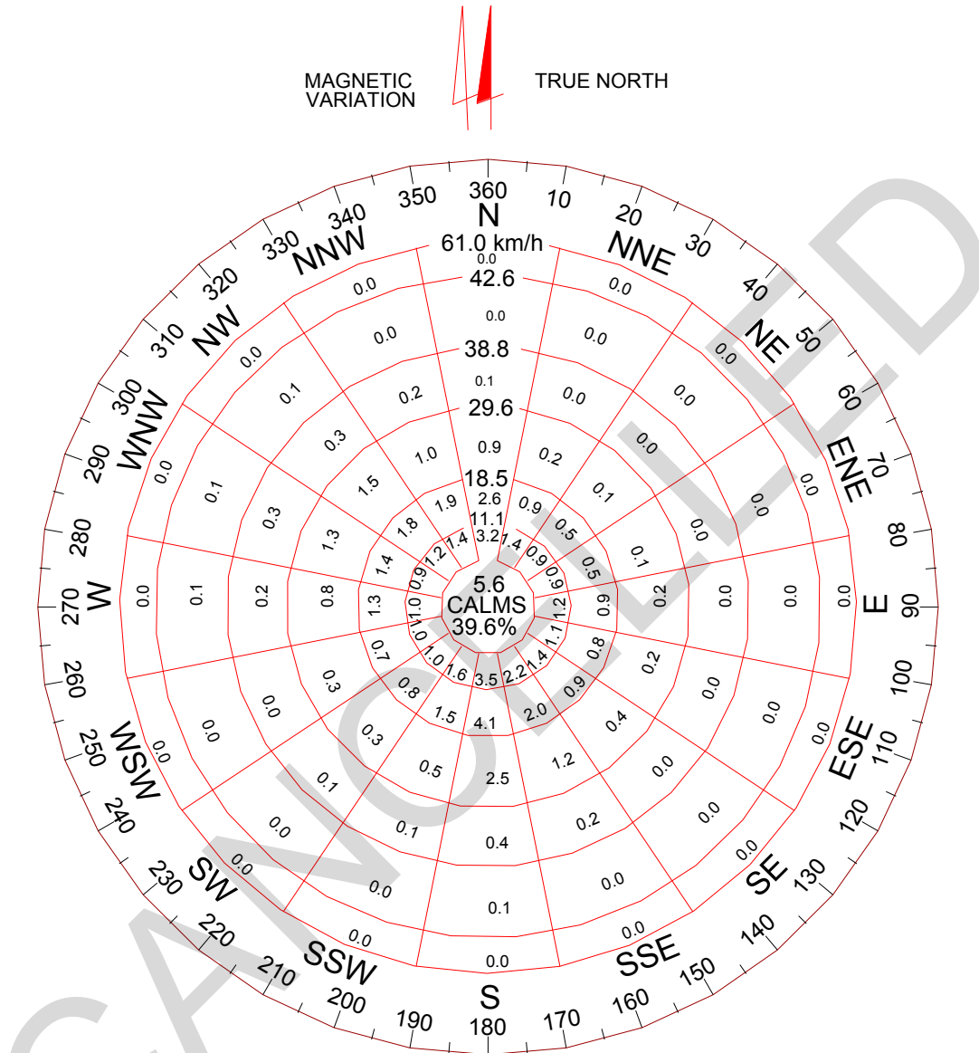
Figure B4-3. Completed Windrose and Wind Velocity Equivalents (16-Sector [22.5°] Windrose)
