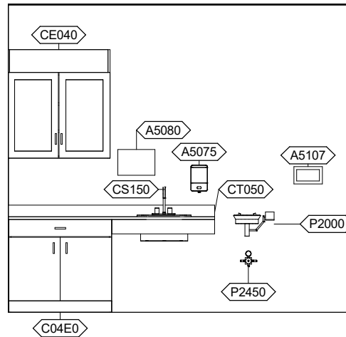
ORSR1 - WEST ELEVATION
