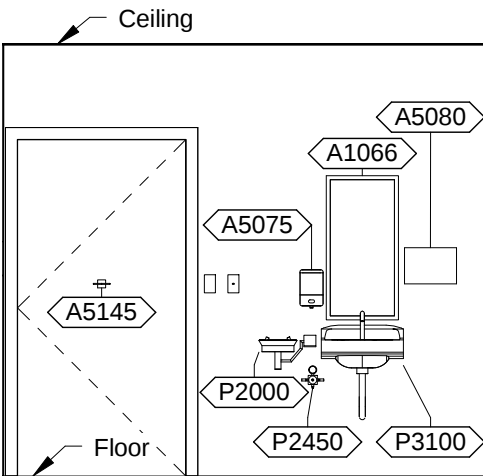
LBVP1 - PLAN SOUTH
