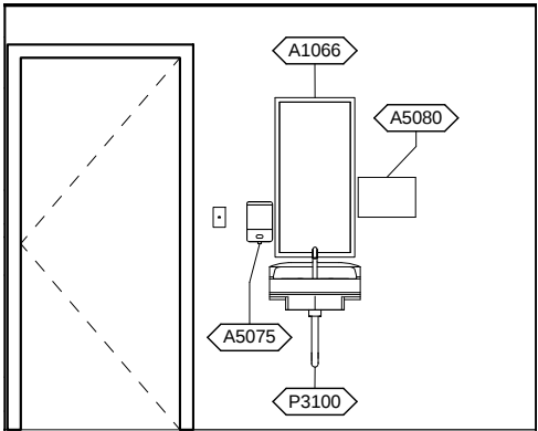
EXRG1 - SOUTH ELEVATION
